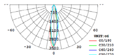
Light Distribution Curve
